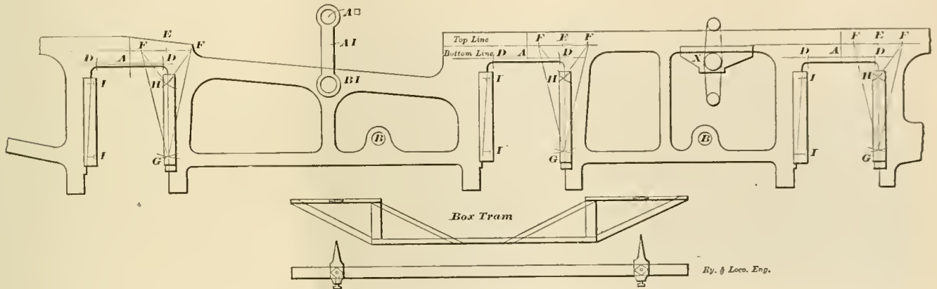
PERCY'S METHOD OF LAYING OFF SHOES AND WEDGES.
